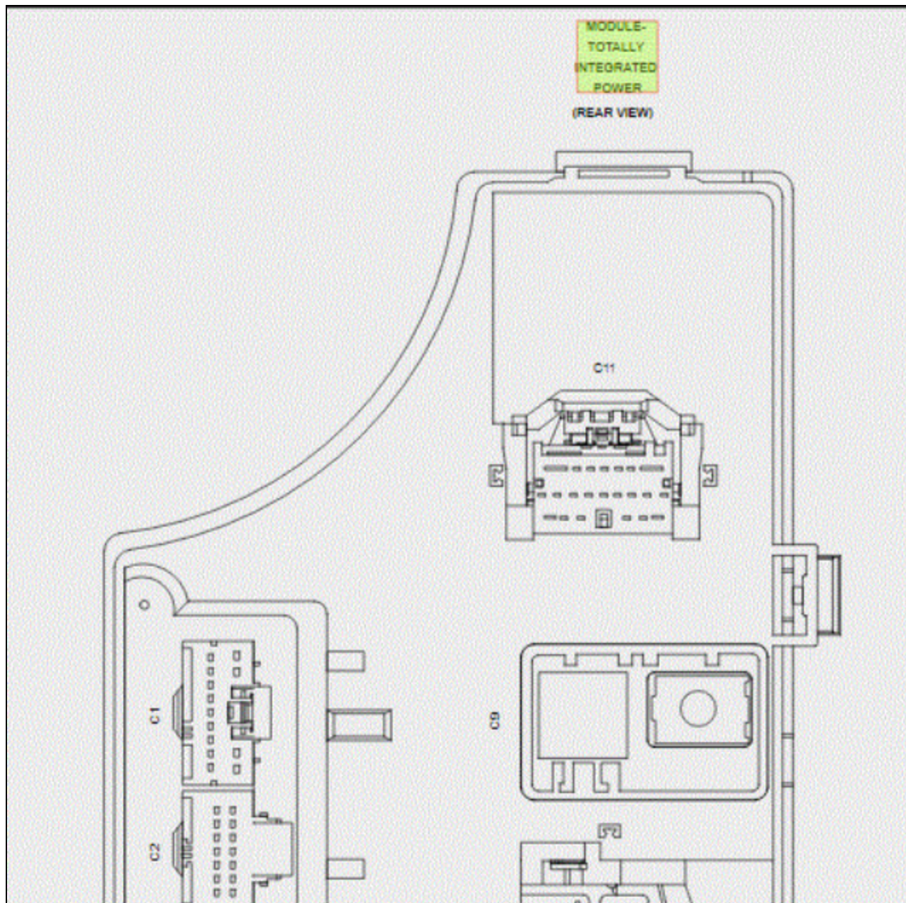
Fig 4: Totally Integrated Power Module Connector Identification
